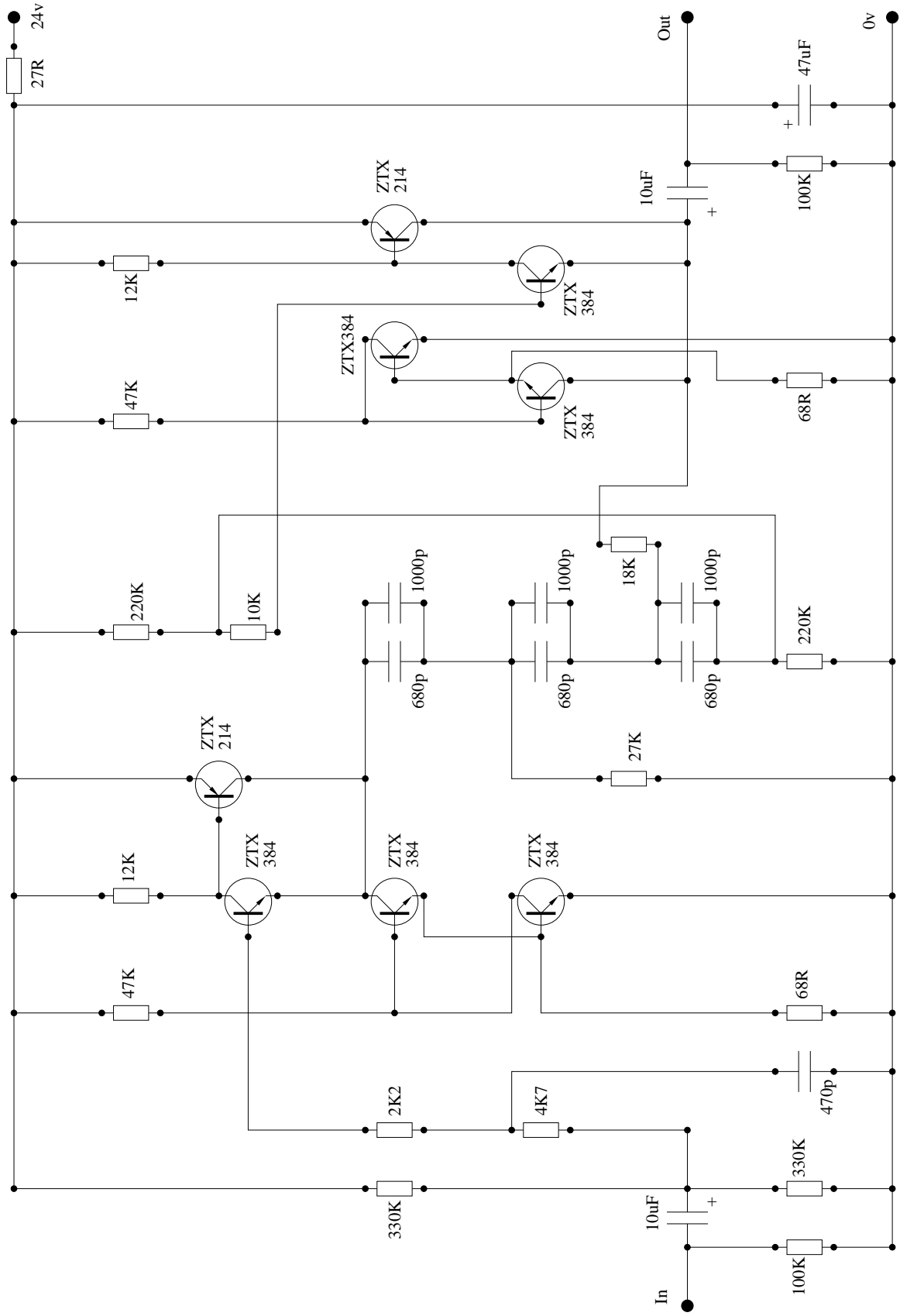
Naim SBL/Kan High Freq Active Crossover Board
